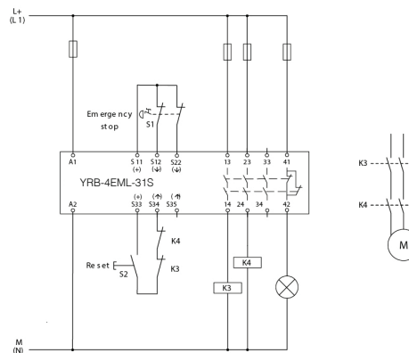
Figure 5 Two-channel emergency stop circuit without cross-circuit detection
