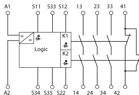
Figure 2 Block diagram
