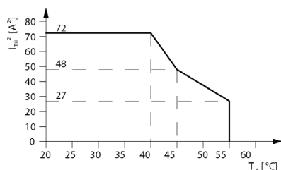
Figure 1 Derating curve
