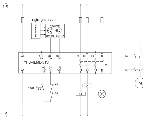
Figure 4 Two-channel light grid monitoring
