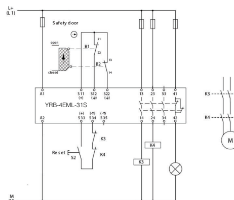
Figure 7 Two-channel safety door monitoring without cross-circuit detection
