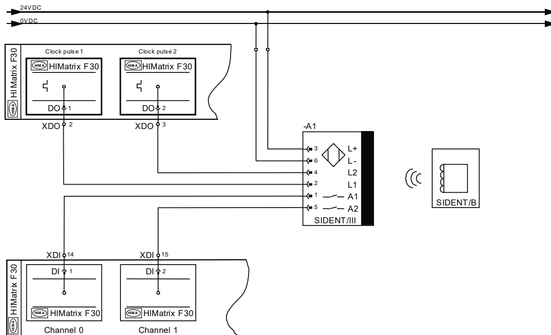
Example for connection: SIDENT/III with safety control (here: HIMA HIMatrix F30)
