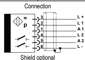
Plug M23 x 1 6-pole, Coninvers RC
