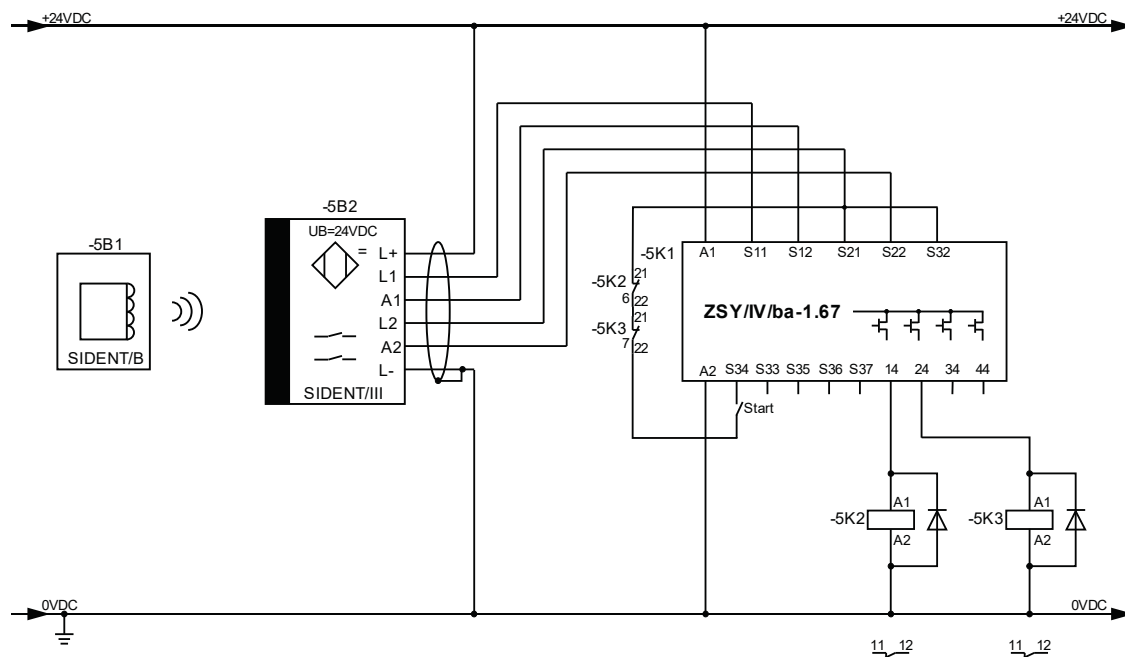
Example for connection: SIDENT/III with safety relay for Safety Switch (here: KLASCHKA ZSY/IV/ba-1.67)
