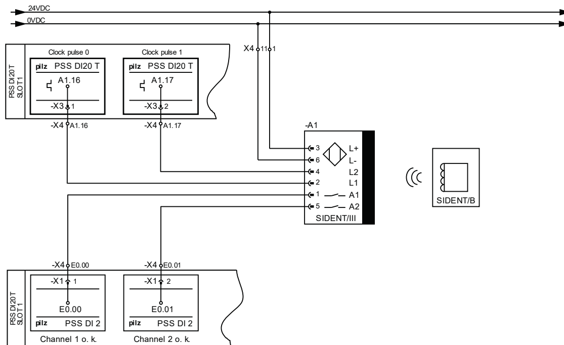
Example for connection: SIDENT/III with safety control (here: PILZ PSS 3000)
