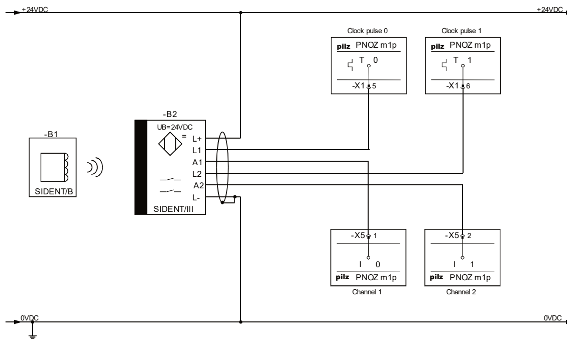
Example for connection: SIDENT/III with safety control (here: PILZ PNOZ multi)
