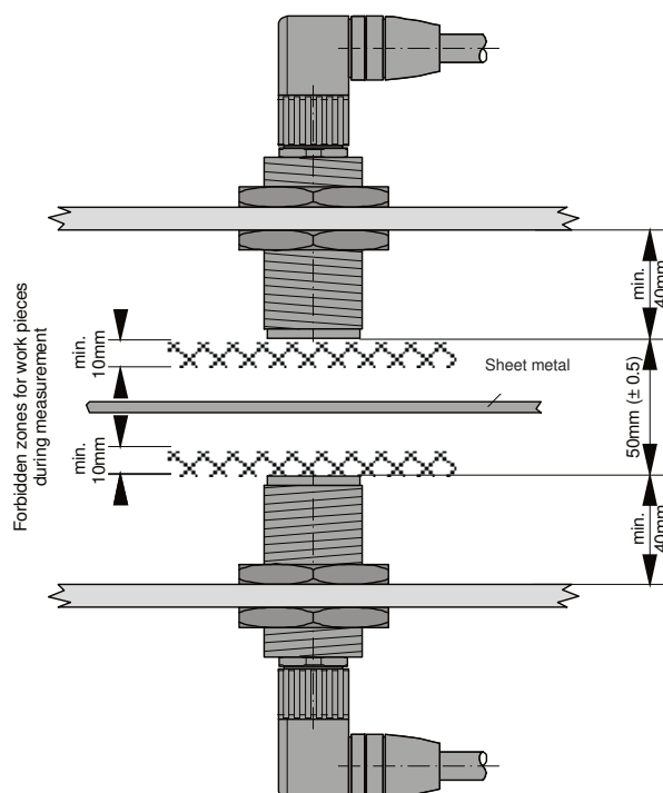
Double surface non-contact measurement with sheet metal thickness sensor pair BDWD/S and BDWD/E.
