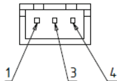
Connector JST - 3-pin / Automatic („HWT2- _6_D...“)
