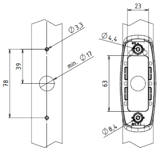
Required drillings on handrail
